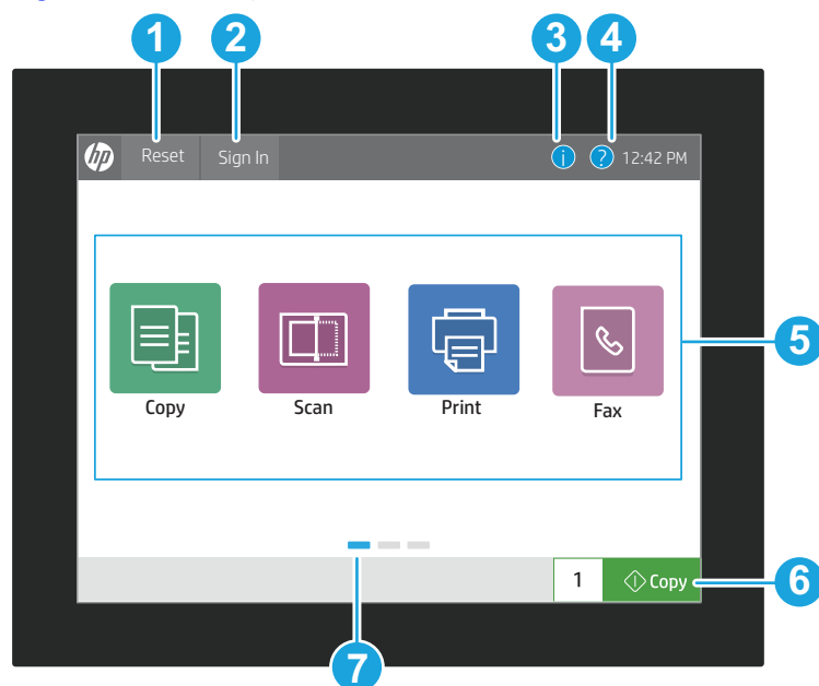
Figure 1-9 Control-panel view
