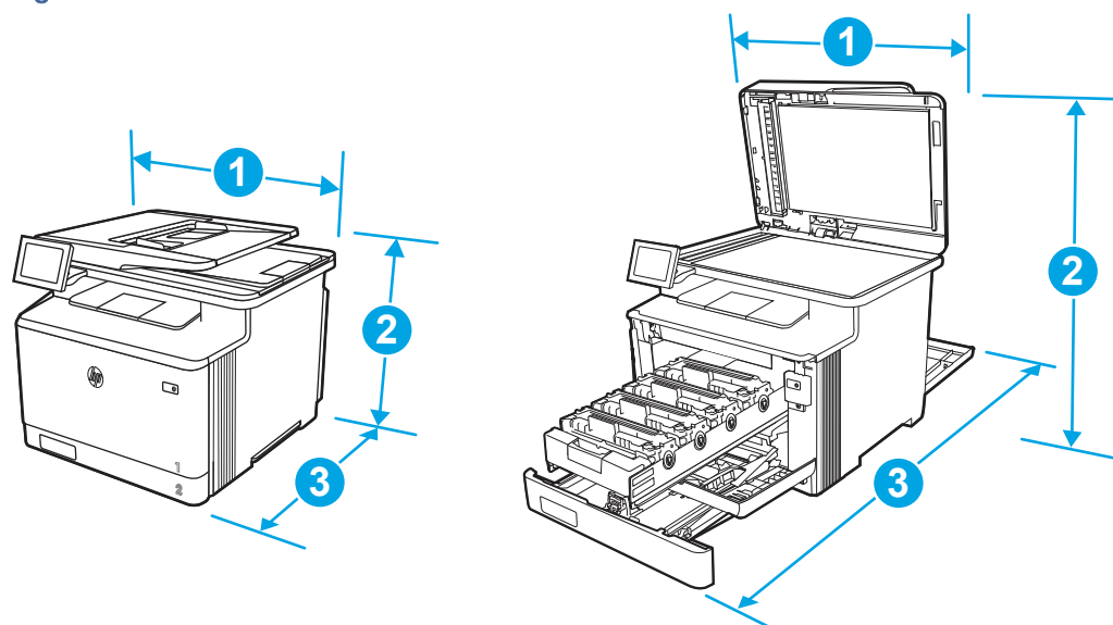
Figure 1-9 Dimensions for the E47528f model
