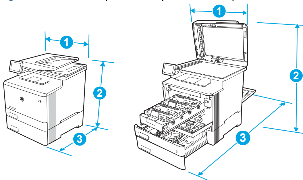
Figure 1-10 Dimensions for the printer with the optional 550-sheet tray
